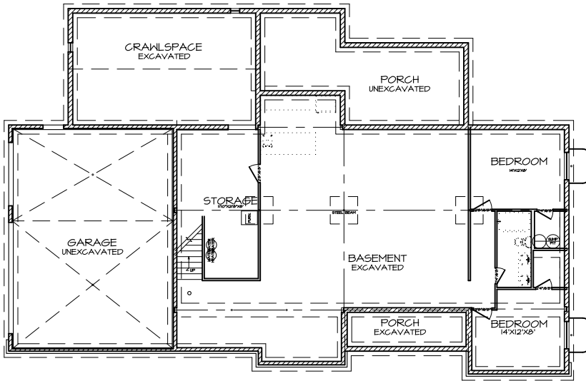
FOUNDATION PLAN A-1
