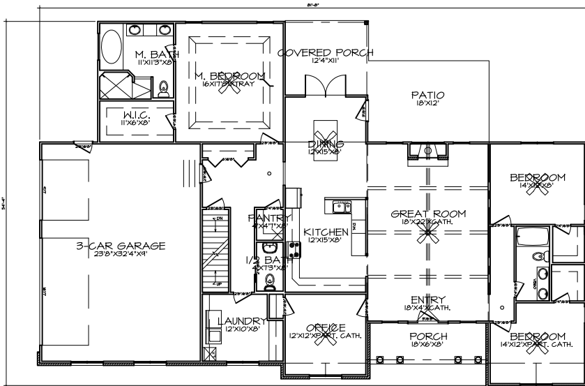
FIRST FLOOR PLAN A-1
